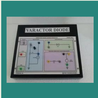
V To I Trainer
